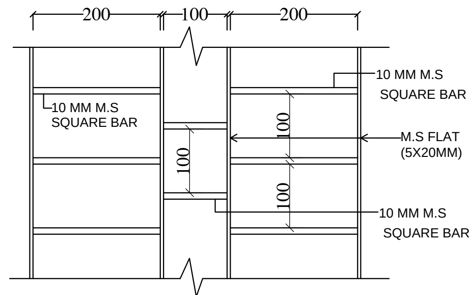
TYPICAL WINDOW AND VENTILATOR GRILL DETAIL
