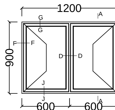
WINDOW TYPE W1
