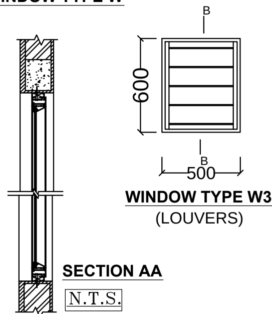
WINDOW TYPE W
