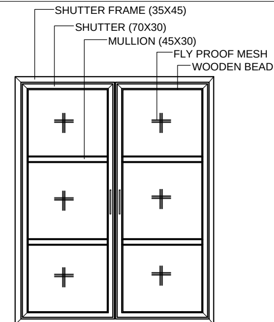
TYPICAL WINDOW AND VENTILATOR FLY PROOF DETAIL
