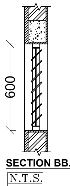
WINDOW TYPE W3 (LOUVERS)
