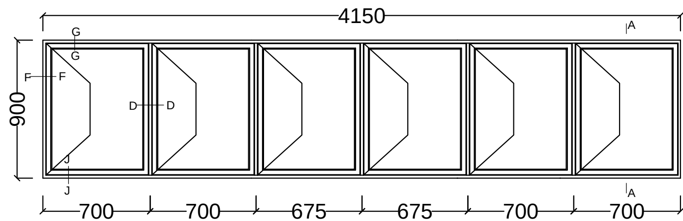
WINDOW TYPE W
