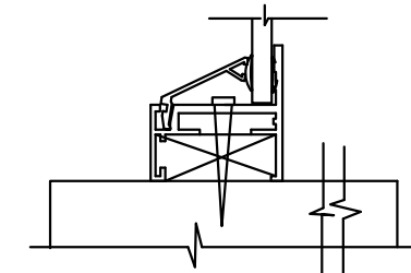
SECTION AT JJ
