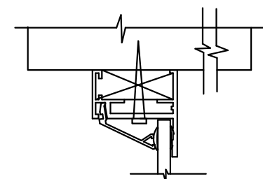
SECTION AT GG
